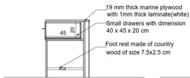
SECTION H
