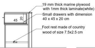
SECTION H
