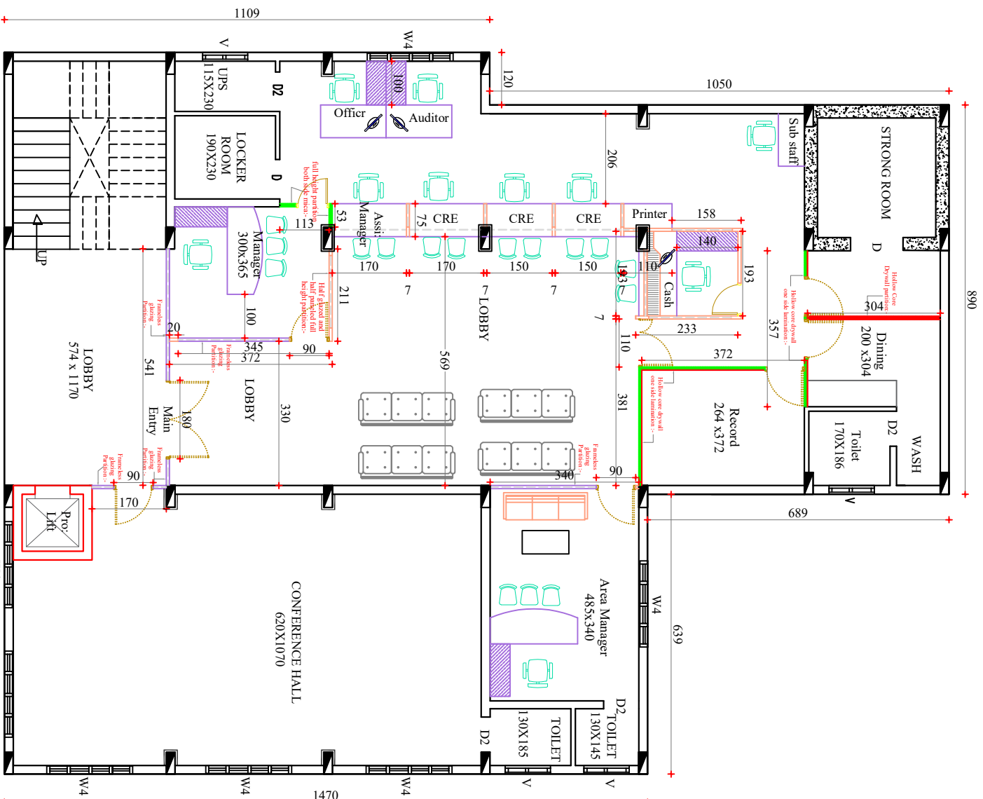
PROPOSED LAYOUT OPTION-2a
